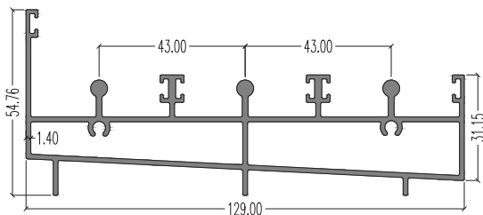
7367 (Bottom Outer) LW : 1.922 kg/m AP : 619.73 mm
