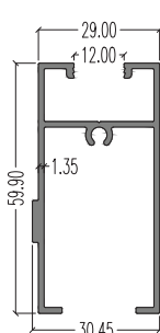
7374 (Bottom Inner) LW : 0.707 kg/m AP : 365.50 mm
