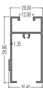
7384 (Bottom Inner) LW : 0.708 kg/m AP : 364.81 mm
