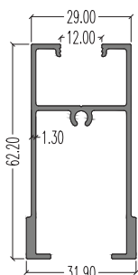
7978 (Bottom Inner) LW : 0.759 kg/m AP : 375.53 mm
