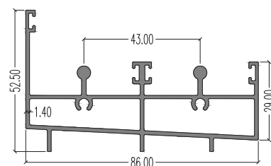
7380 (Bottom Outer) LW : 1.343 kg/m AP : 449.00 mm
