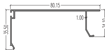
7971 (Capping) LW : 0.461 kg/m AP : 296.72 mm (For 7376, 7371 & 5094)
