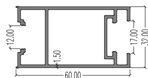
5087 (Side Inner) LW : 0.912 kg/m AP : 311.28 mm (For Multipoint Locking)
