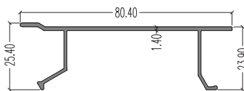
7387 (Capping) LW : 0.474 kg/m AP : 271.99 mm (For 7372)
