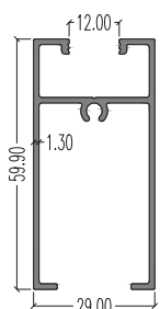
7966 (Bottom Inner) LW : 0.652 kg/m AP : 362.31 mm
