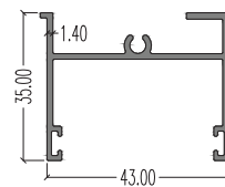
7381 (Top & Side Outer) LW : 0.509 kg/m AP : 282.53 mm (For 7379 & 7977)
