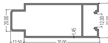
7936 (Intermediate) LW : 0.953 kg/m AP : 301.91 mm (For 7935)
