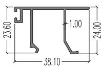
7370 (Capping) LW : 0.306 kg/m AP : 202.44 mm (For 7373, 7376, 5080 & 5094)
