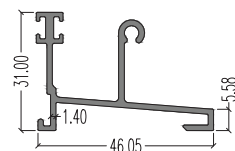
7922 (Bottom Outer) LW : 0.548 kg/m AP : 278.70 mm (For 7970)
