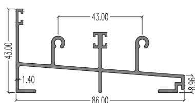
7970 (Bottom Outer) LW : 1.012 kg/m AP : 508.33 mm
