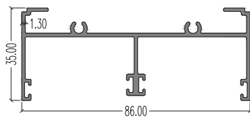
7977 (Top & Side Outer) LW : 0.831 kg/m AP : 466.95 mm
