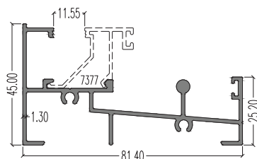
5080 (Bottom Outer) LW : 0.941 kg/m AP : 492.32 mm
