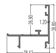
46916 (Attachment Beading) LW : 0.333 kg/m AP : 215.22 mm
