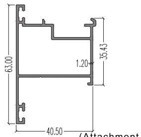
46903 (Attachment Inner) LW : 0.694 kg/m AP : 282.94 mm
