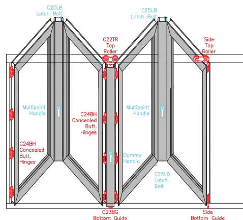
Interior View
