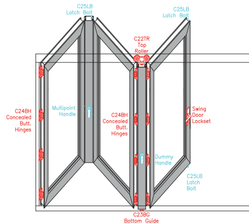
Interior View
