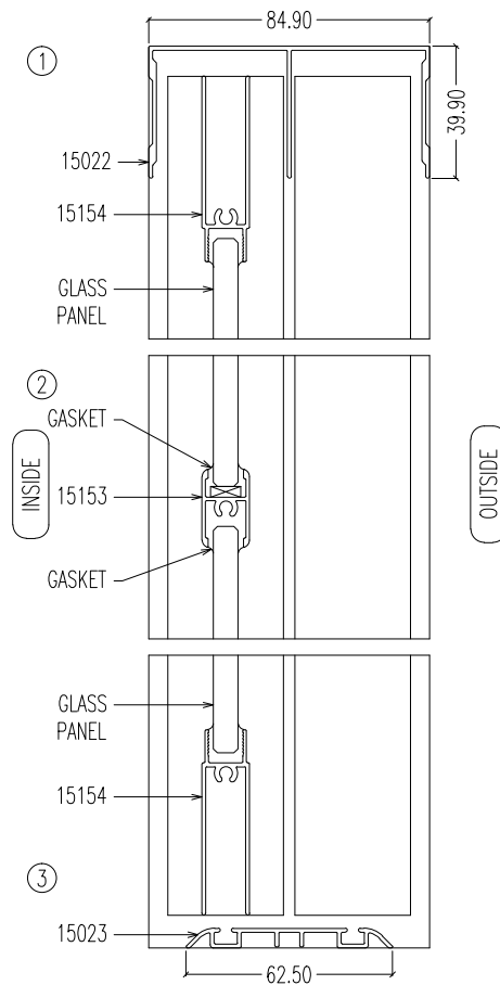
VERTICAL SECTIONS
