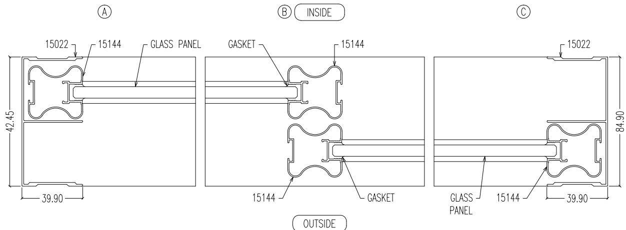
HORIZONTAL SECTIONS
