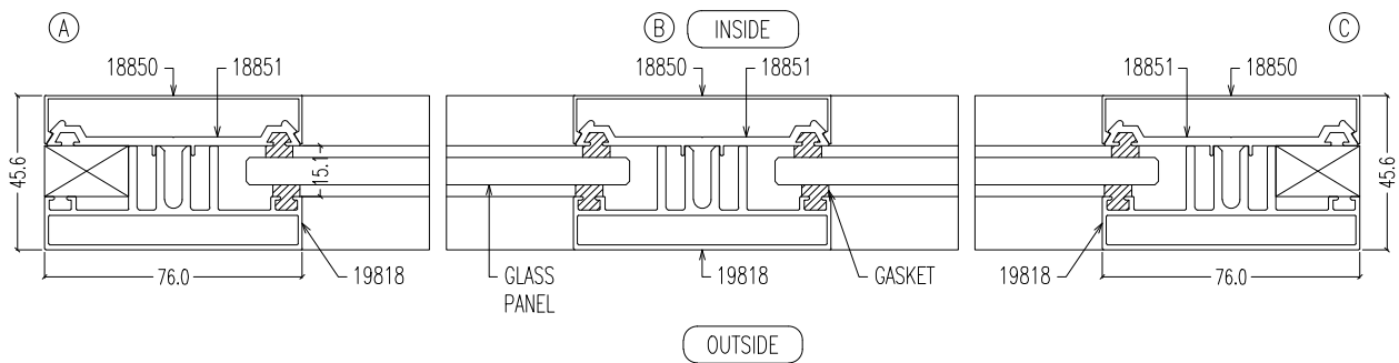
VERTICAL SECTIONS
