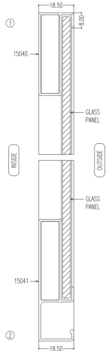
VERTICAL SECTIONS
