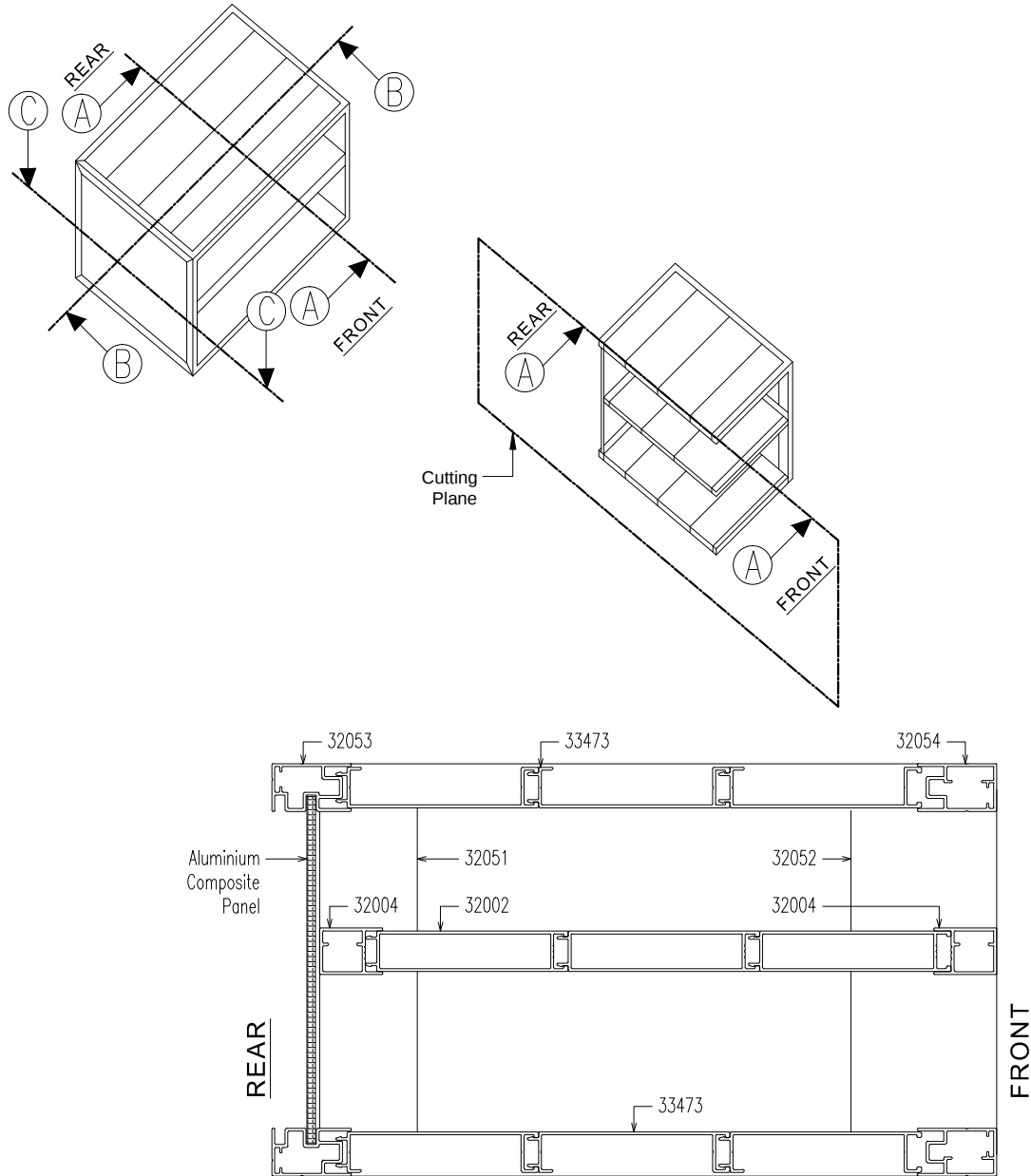
SECTIONAL VIEW A-A
