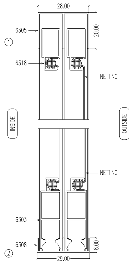
VERTICAL SECTIONS
