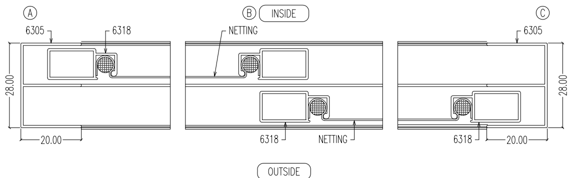
HORIZONTAL SECTIONS
